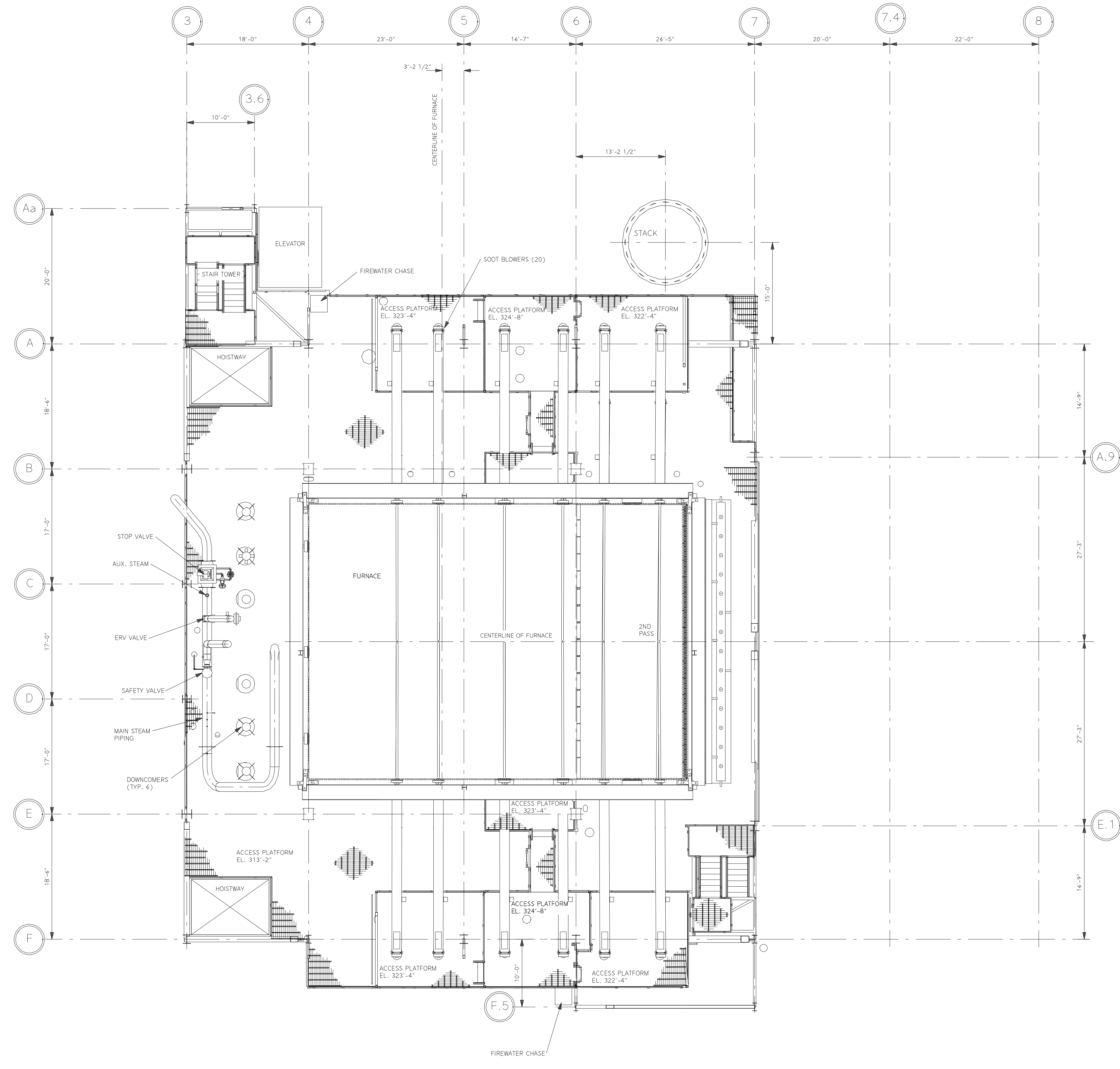
PLAN VIEW ELEVATION 313'-2", 322'-4", 323'-4", 324'-8"
